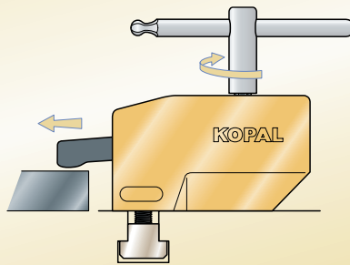
Extension of the arm
