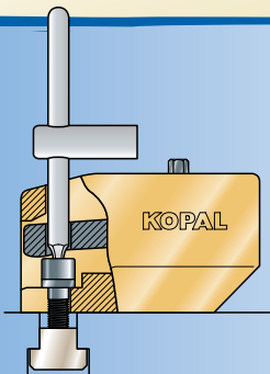
Simple and quick fixing with M 10 screw (provided)
