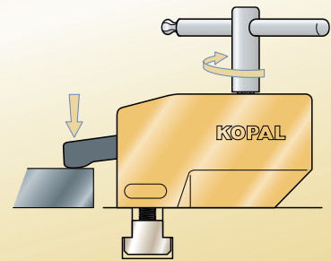
Clamping of the workpiece
