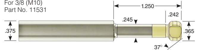
Loc-Down® 1/2" Carbide Cutter For 1/2 (M12) and 5/8 (M16) Part No. 11530
