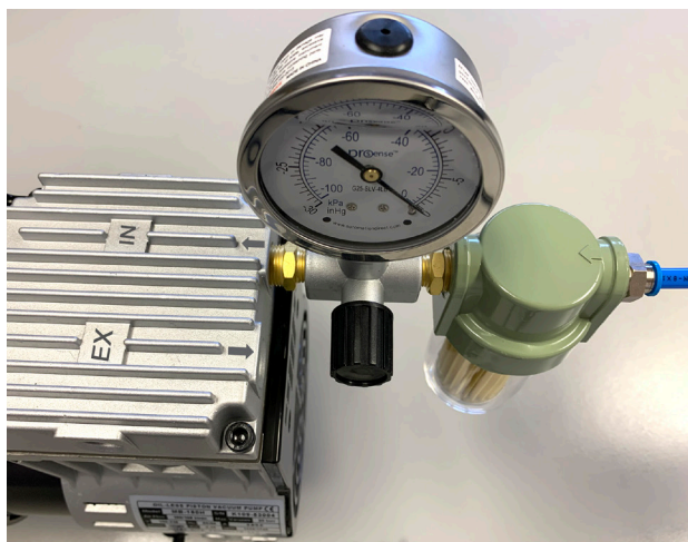
Vacuum Port set-up
