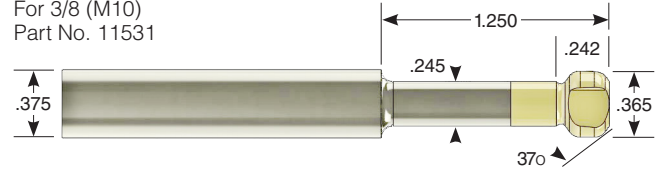
Loc-Down® 1/2" Carbide Cutter For 1/2 (M12) and 5/8 (M16) Part No. 11530
